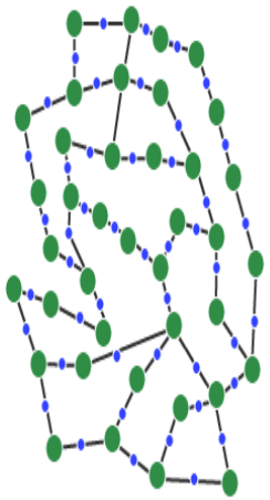
Amorphous Solids
