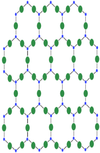
Crystalline Solids
